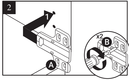
2. Attach mounting plate (A) to cabinet with screw (B).
